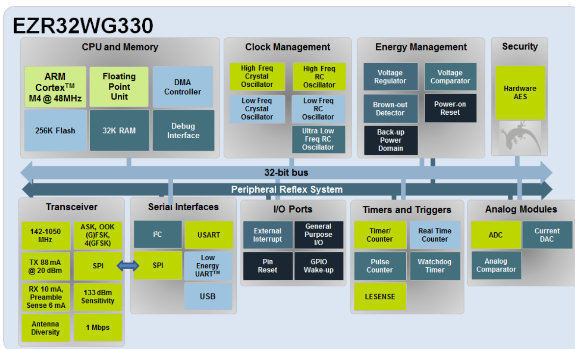
Figure 3.1. Block Diagram
